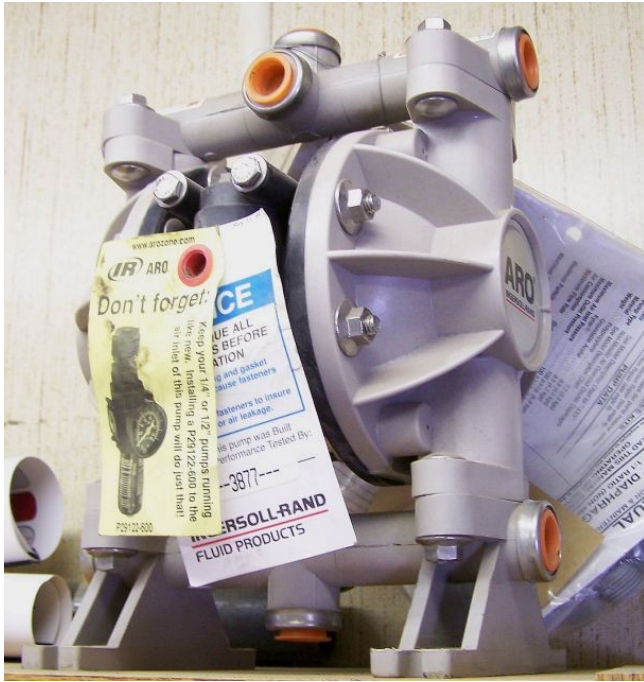
New Ingersoll-Rand Diaphragm Pump. 1/2 in.
