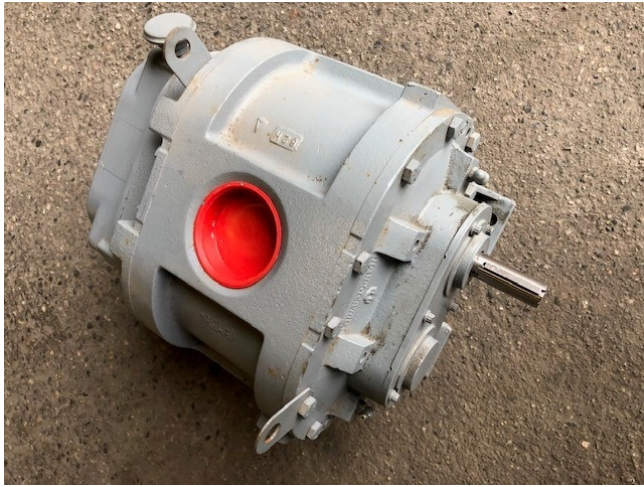
Sutorbilt 3LP Positive Displacement Blower
