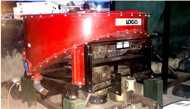
Kelsey J1300 Centrifugal Mineral Jig
