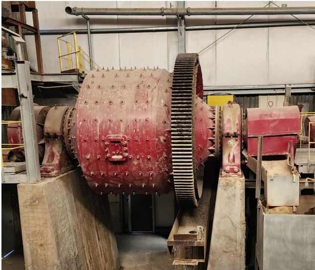
Hardinge 10ft Dia. x 5ft Long Conical Ball Mill
