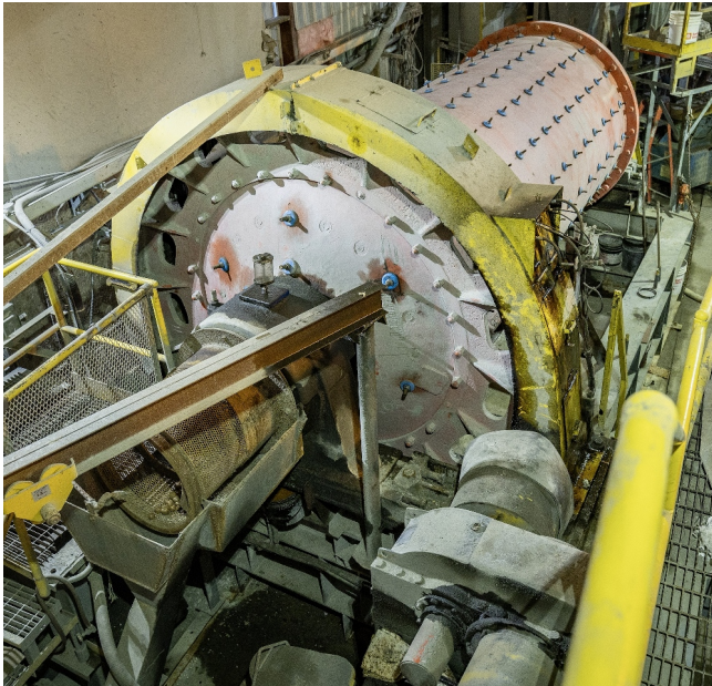
Allis Chalmers 5ft Dia. x 16ft Long Ball Mill
